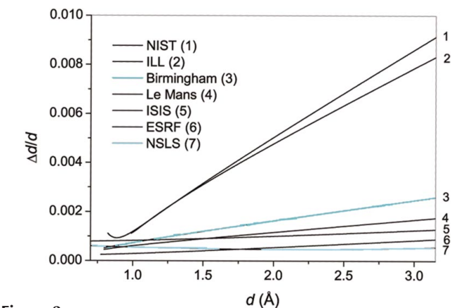
Figure 2 Resolution function \Delta d/d as a function of interplanar spacing d for all instruments, as calculated from the FWHM obtained by Rietveld refinement, for the sample S2.
