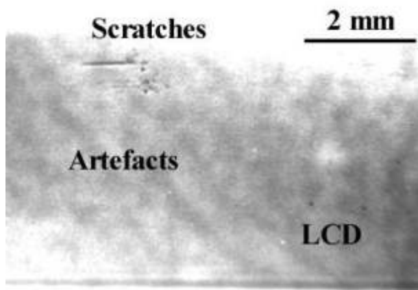
Fig. 3. Monochromatic projection topography of a 80 \mu\text{m} thick Si wafer (grounded and etched).
