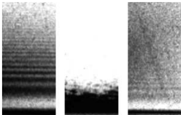
Fig. 2. Sub-surface damage characterisation by Pendellösung fringes visibility: reference Si wafer (left), ground wafer (middle), ground and 46 \mu\text{m} etched wafer (right).
