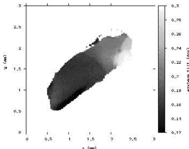
Fig. 4. Distribution of maximum of the lateral lattice misorientation angle onto a defective area of a GaAs wafer.
